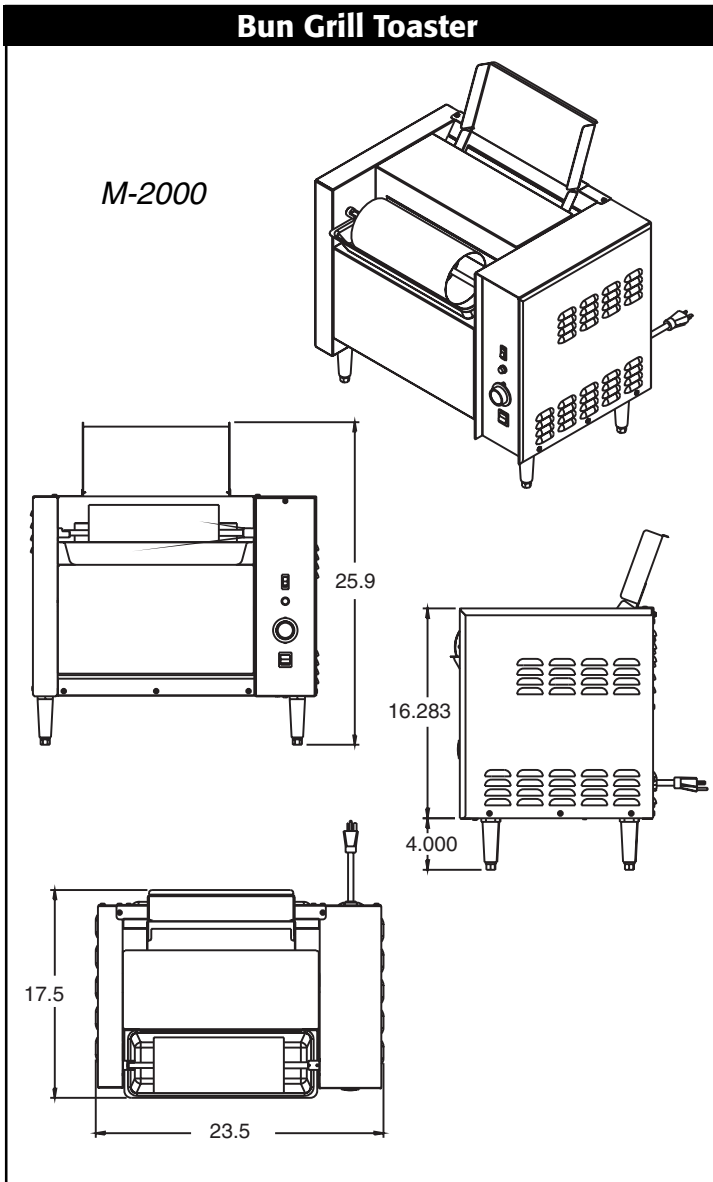
Model M-2000 Bun Grill Toaster
